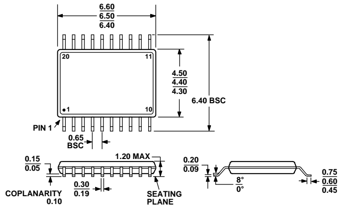
COMPLIANT TO JEDEC STANDARDS MO-153-AC Figure 51. 20-Lead Thin Shrink Small Outline Package [TSSOP] (RU-20) Dimensions shown in millimeters
