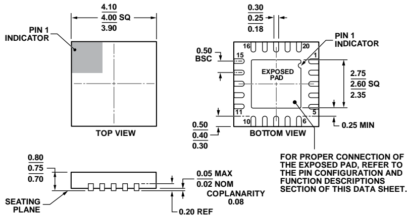
COMPLIANT TO JEDEC STANDARDS MO-220-WGGD. Figure 52. 20-Lead Lead Frame Chip Scale Package [LFCSP] 4 mm x 4 mm Body and 0.75 mm Package Height (CP-20-8) Dimensions shown in millimeters
