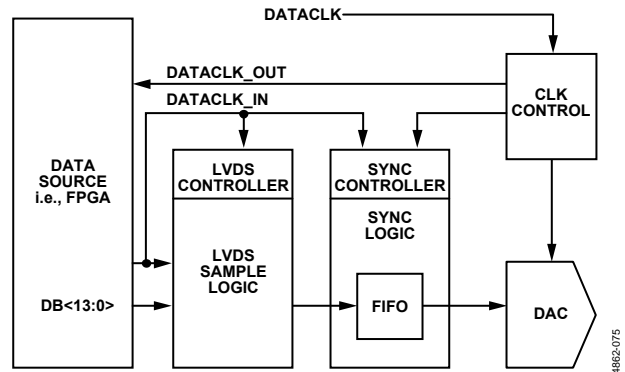
Figure 77. Data Controllers
