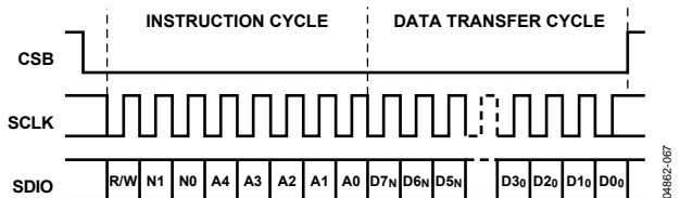
Figure 69. Serial Register Interface Timing, MSB-First Write
