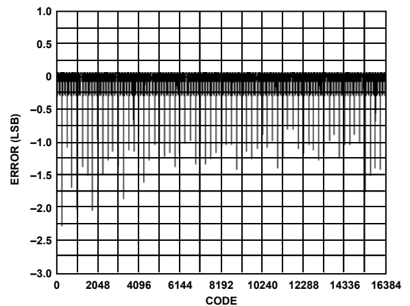
Figure 26. AD9736 DNL, 85°C, 30 mA FS
