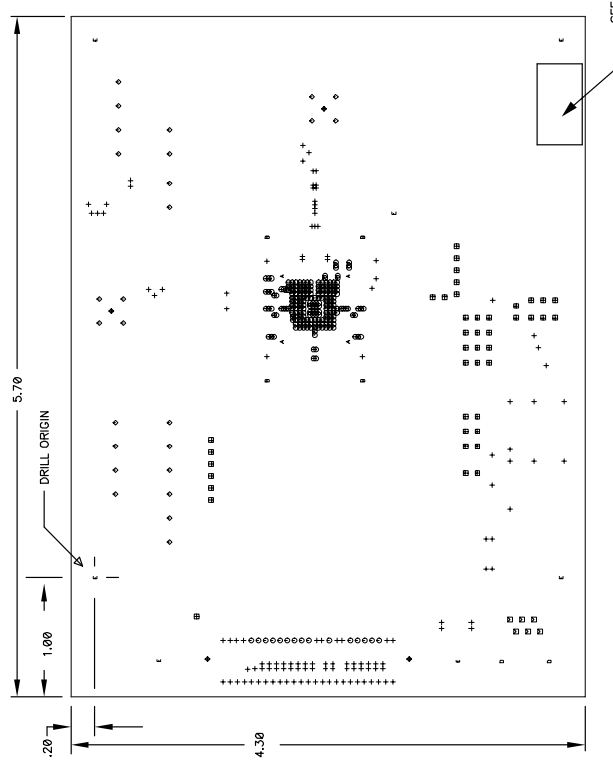
Figure 115. PCB Fabrication Detail, AD973x Evaluation Board, Rev. F
