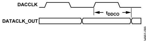
Figure 101. DACCLK to DATACLK_OUT Delay
