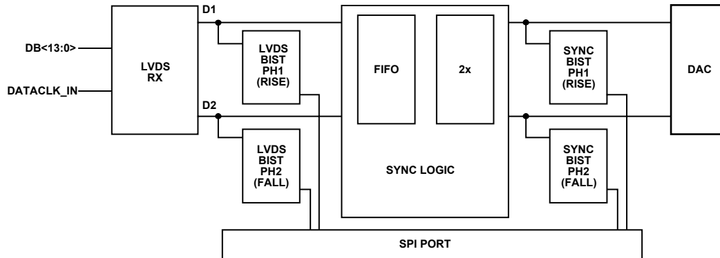
Figure 84. Block Diagram Showing LVDS and SYNC Phase 1 and SYNC Phase 2
