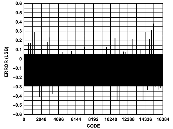
Figure 24. AD9736 DNL, -40°C, 30 mA FS
