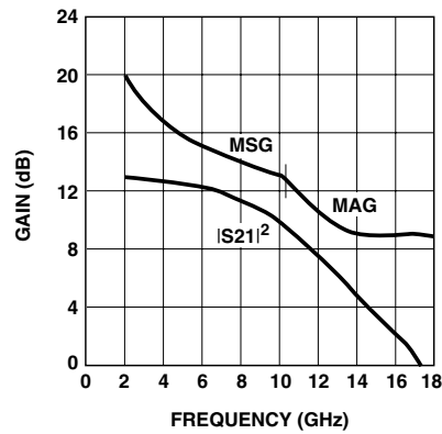
Figure 4. Maximum Available Gain, Maximum Stable Gain & Insertion Power Gain vs. Frequency for V_{DS} = 1.5 V , I_D = 15 mA .
