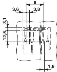
Drilling diagram
