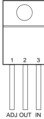
3-Lead Plastic TO-220 \theta_{JC} = 3^{\circ}\text{C/W}
