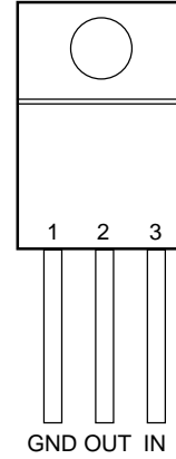
3-Lead Plastic TO-220 \theta_{JC} = 3^{\circ}\text{C/W}
