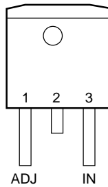
3-Lead Plastic TO-263 Center Cut \theta_{JC} = 3^{\circ}\text{C/W}^*
