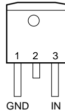
3-Lead Plastic TO-252 \theta_{JC} = 3^{\circ}\text{C/W}^*
