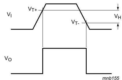
Fig 6. Definitions of V_{T+} , V_{T-} and V_H
